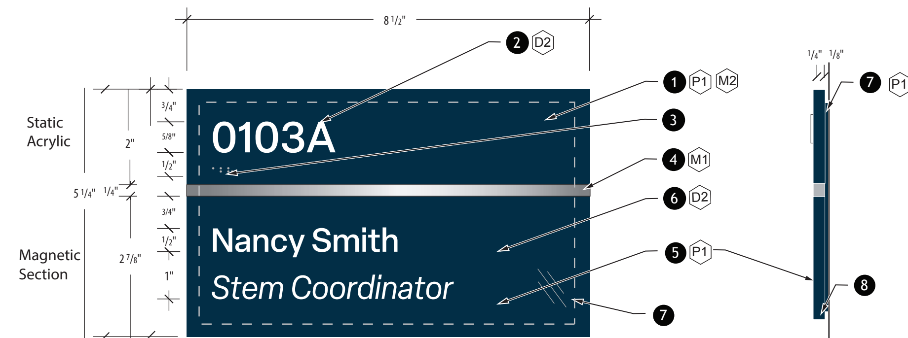
1 FRONT VIEW DETAIL SCALE: HALF ACTUAL SIZE
