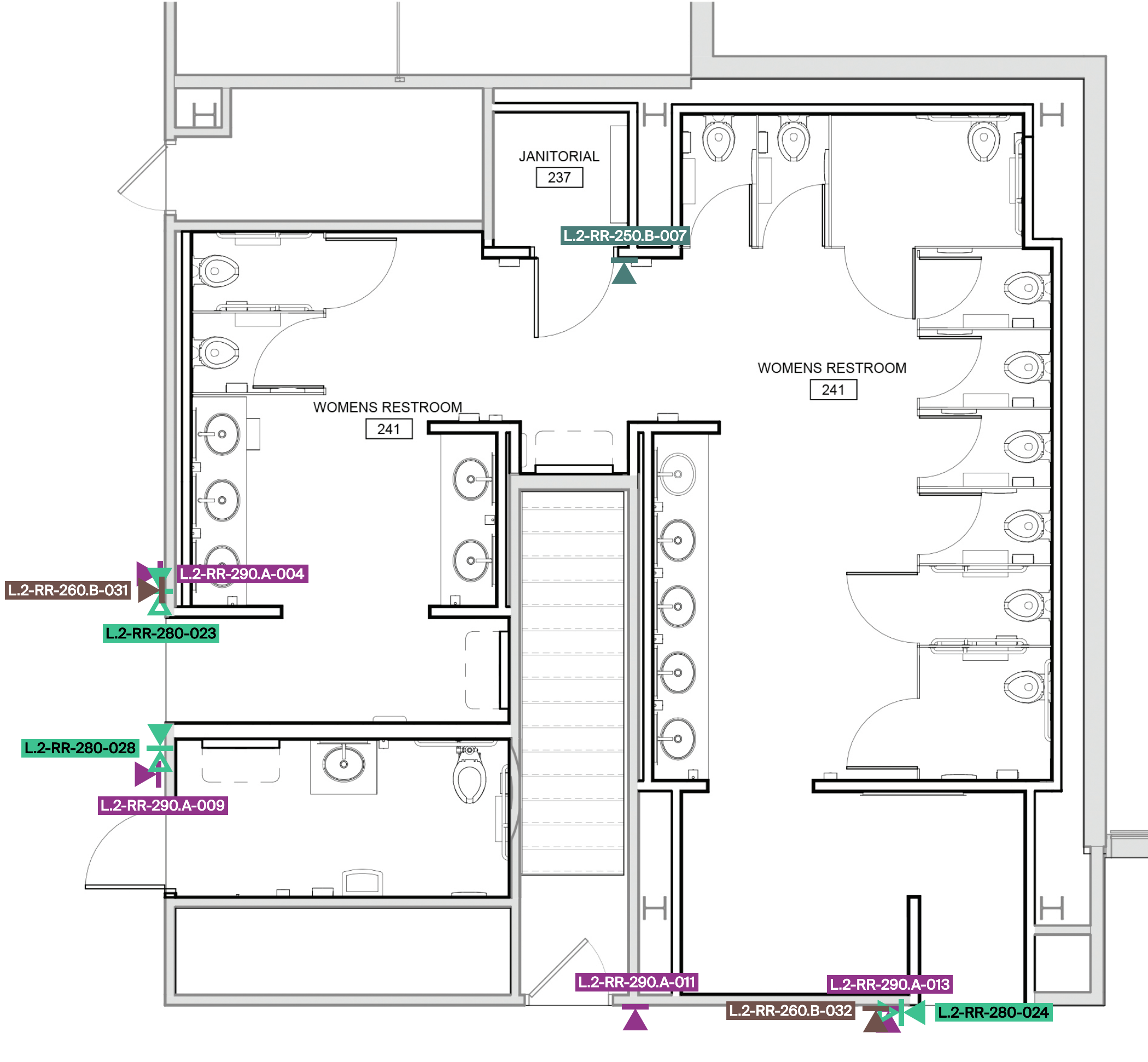
2 WOMENS RESTROOM 241 & MULTI-USER RESTROOM 241A - SIGNAGE PLAN 1/4" = 1'-0"
