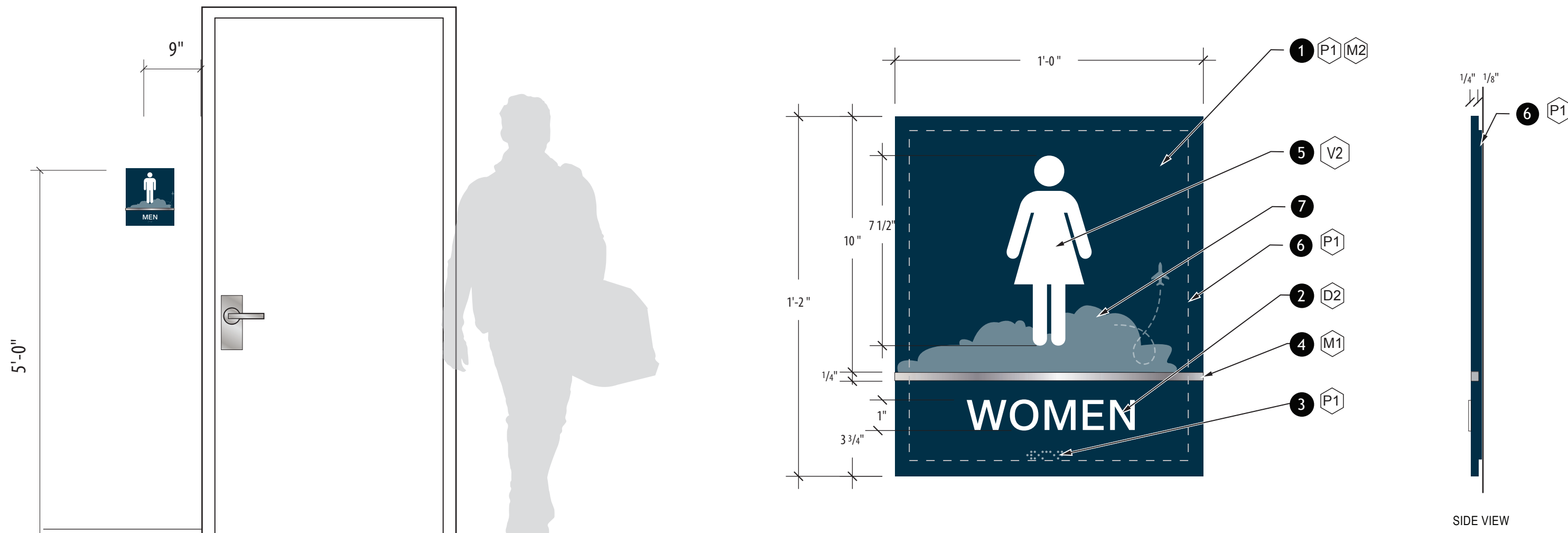
1 ST 290.A: ADA STAIR / RESTROOM IDENTIFICATION, ELEVATION SCALE: 3/4" = 1'
