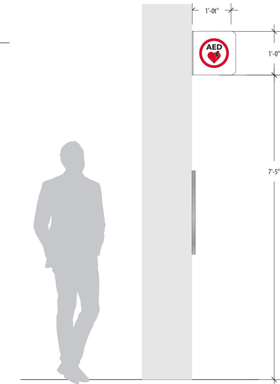
3 ST 330- FIRE LIFE SAFETY FLAG, DETAIL SCALE: 3/4" = 1'- 0"
