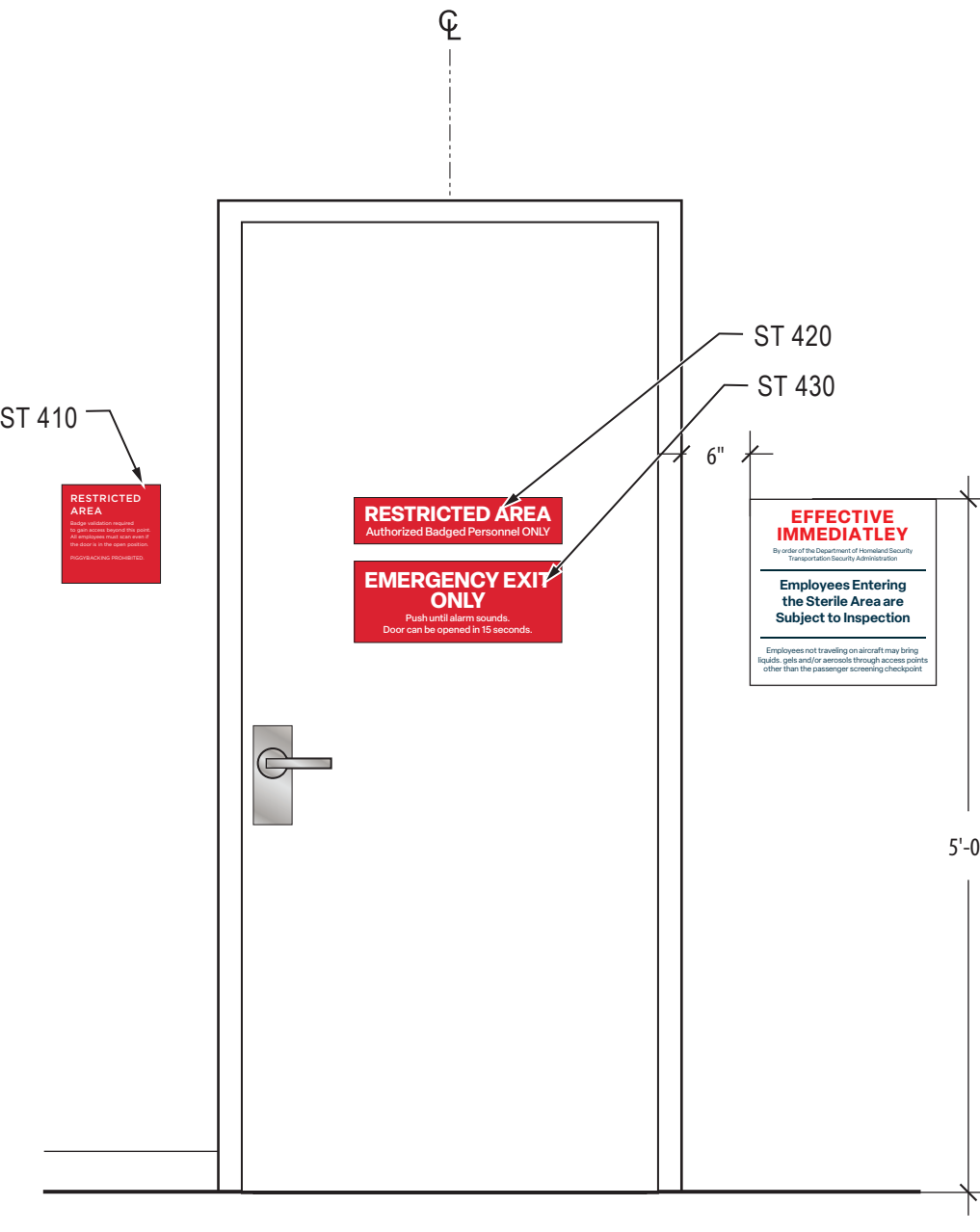
ELEVATION AT STAIR 4 (B203/B205)
