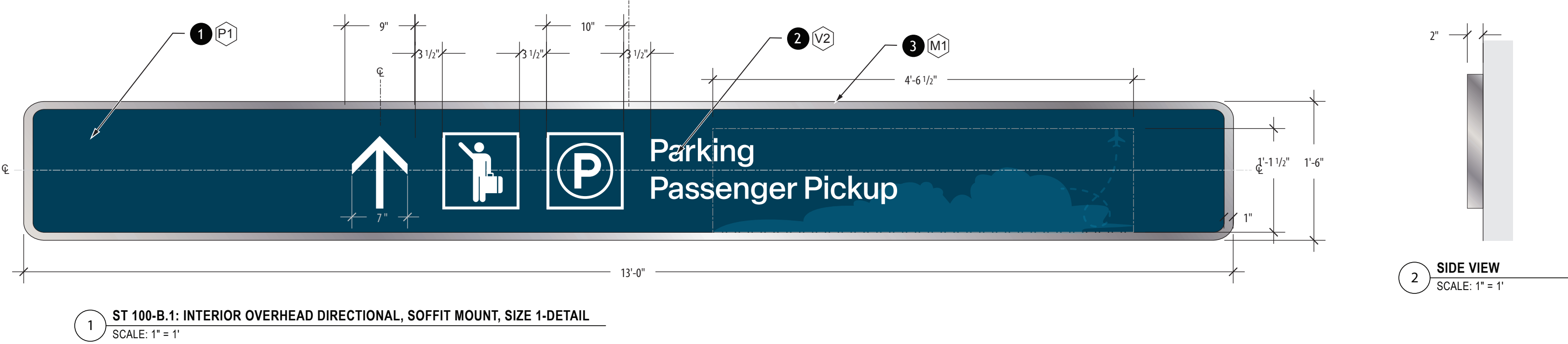
1 ST 100-B.1: INTERIOR OVERHEAD DIRECTIONAL, SOFFIT MOUNT, SIZE 1-DETAIL SCALE: 1" = 1'
