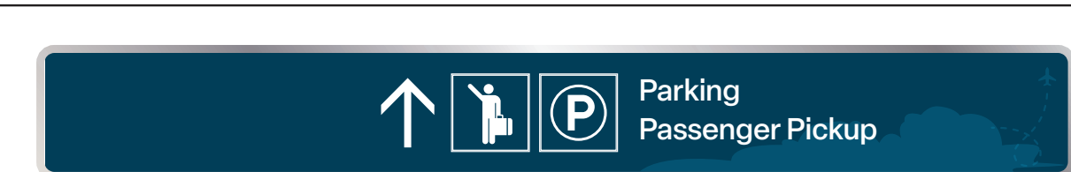
1 ST 100-B.1: INTERIOR OVERHEAD DIRECTIONAL, SOFFIT MOUNT, SIZE 1-DETAIL SCALE: 1" = 1'
