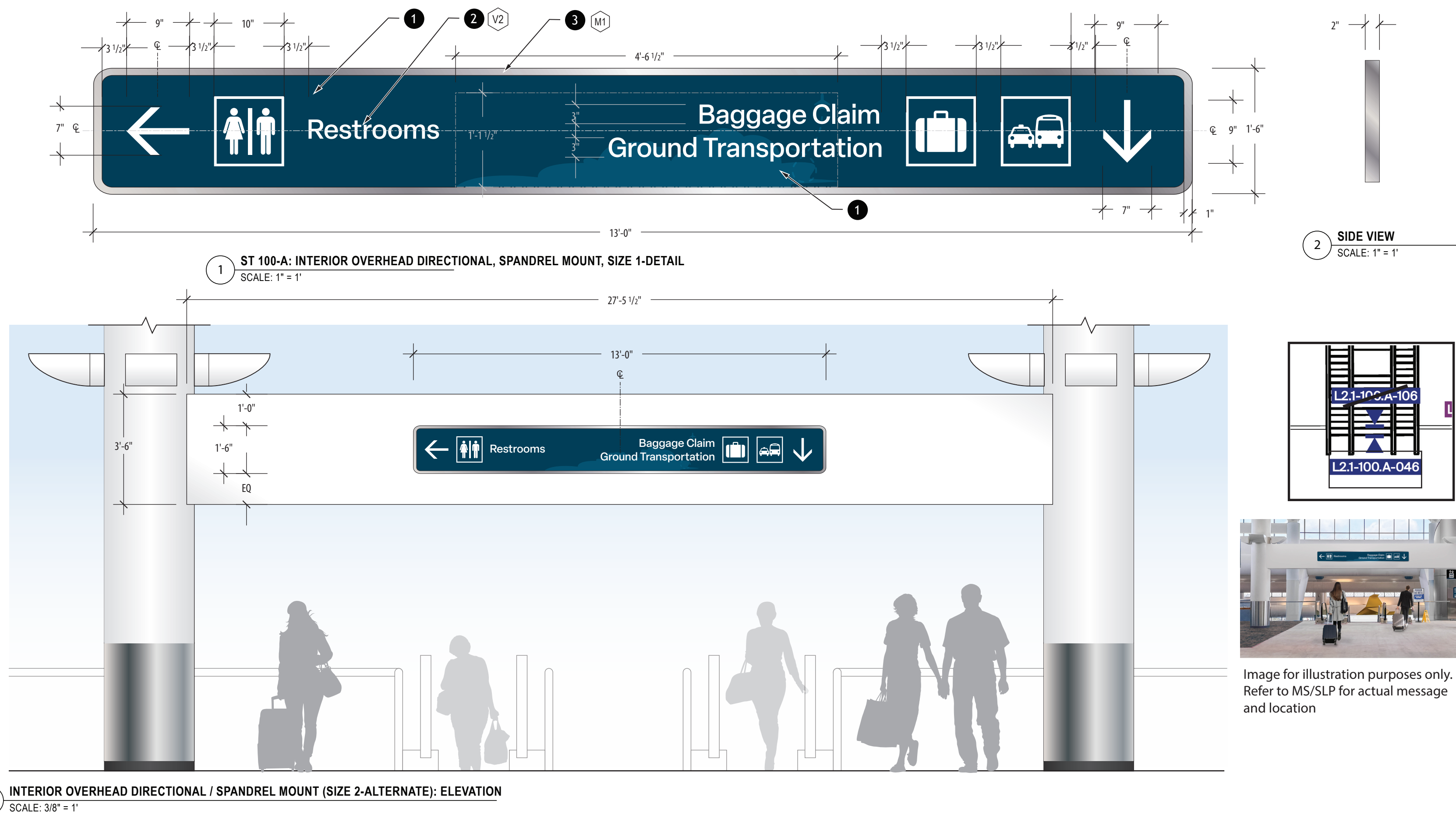
1 INTERIOR OVERHEAD DIRECTIONAL / SPANDREL MOUNT (SIZE 2-ALTERNATE): ELEVATION SCALE: 3/8" = 1'
